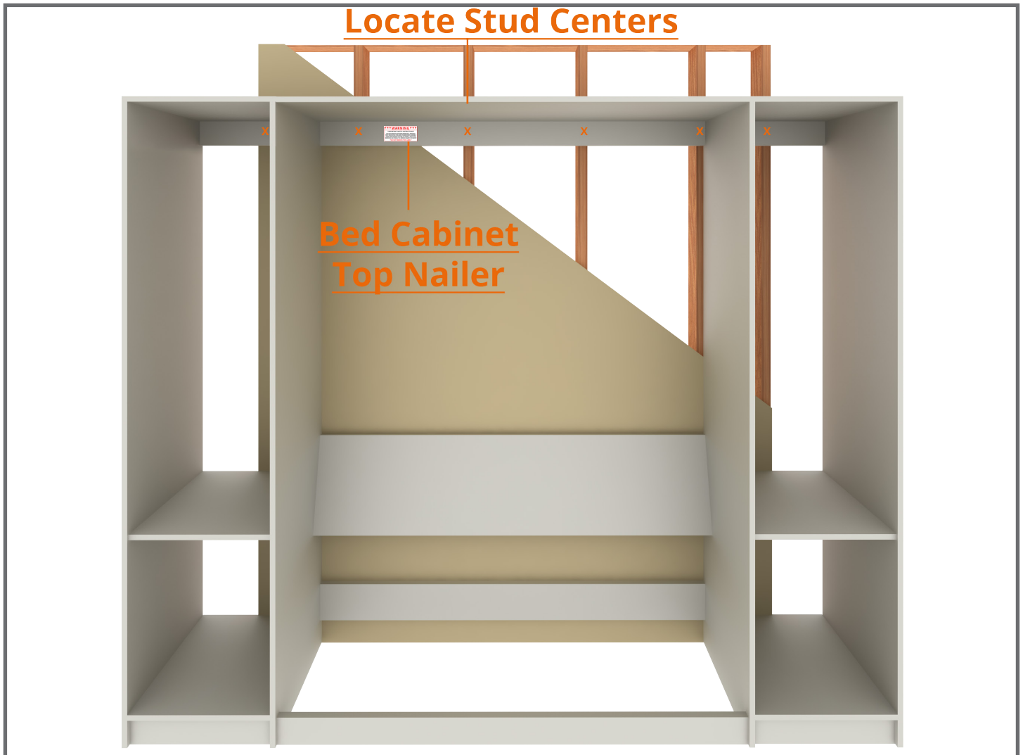
FIG. 3A - DRYWALL CUTAWAY SHOWING WALL STUDS
