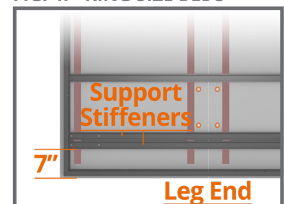
FIG. 4I - KING SIZE BEDS
